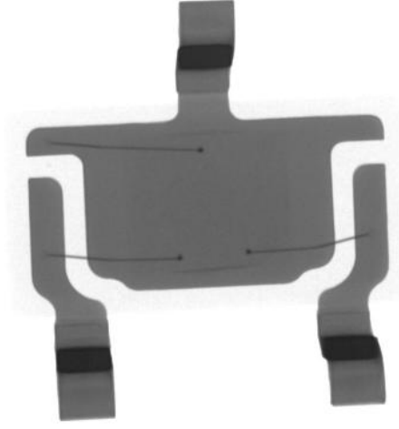
#8-Top View-All
