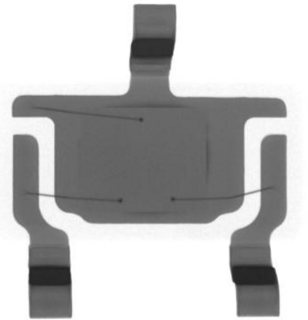
#4-Top View-All
