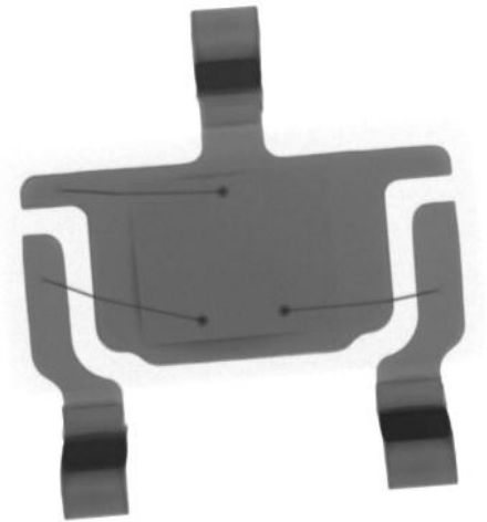
#7-Top View-All
