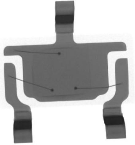
#5-Top View-All
